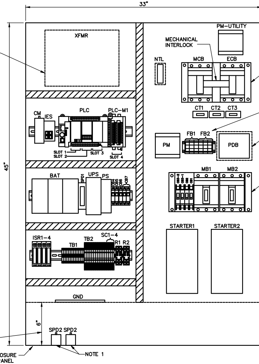
ENCLOSURE INTERIOR SUBPANEL LAYOUT
